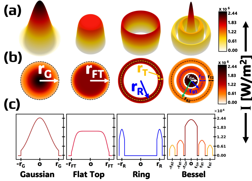
Figure 3: Visualization of four laser beam profiles- Gaussian, Flat-Top, Ring, and Bessel, used for laser-aided phase-field simulations of unary Au. (a) 3D intensity maps of the four beam types, each with an equivalent outer radius of 70\mu m . The peak intensities at the beam center are 2.44 \times 10^6 W/m^2 for Gaussian, 1.58 \times 10^6 W/m^2 for Flat-Top, 1.70 \times 10^6 W/m^2 for Ring, and 2.33 \times 10^6 W/m^2 for Bessel beam, as shown by the color scale. (b) Top-view intensity distributions for the same beams, where r_G and r_{FT} denotes the Gaussian and Flat-Top beam radii, respectively, and r_R and r_T indicates the Ring beam radius and thickness. For the Bessel beam with a central core and two outer rings, the core radius is r_{G0} , while the outer rings have radii r_{R1} and r_{R2} with respective thickness r_{T1} and r_{T2} . (c) Side-view irradiance profile showing the variation of intensity with radial distance, where the y-axis represents irradiance and the x-axis represents the distance from the beam center.
