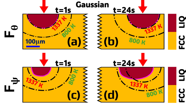
Figure 5: Phase evolution in a unary Au system irradiated by a Gaussian laser beam ( 25 \text{ mW} , 30 \mu\text{m/s} ) scanning from the top left to the top right of the computational domain. Subplots (a) and (b) shows phase-field simulations using the fine-tuned free energy expression ( F_\theta ) at t = 1\text{s} and t = 24\text{s} , respectively, where the LIQUID phase (dark red) aligns with the melting temperature contour of 1337 \text{ K} . Subplots (c) and (d) presents results using the TDB-based free energy expression ( F_\psi ), indicating a time lag between thermal and phase diffusion, with thermal diffusion leading. At t = 1\text{s} , the melt pool is 18484.18 \mu\text{m}^2 for F_\theta and 7575.42 \mu\text{m}^2 for F_\psi , which converge to an average of \approx 17800 \mu\text{m}^2 by the end of the simulation, though the melt pool shape differ significantly. Results for Flat-Top, Ring and Bessel beam are provided in Appendix A
