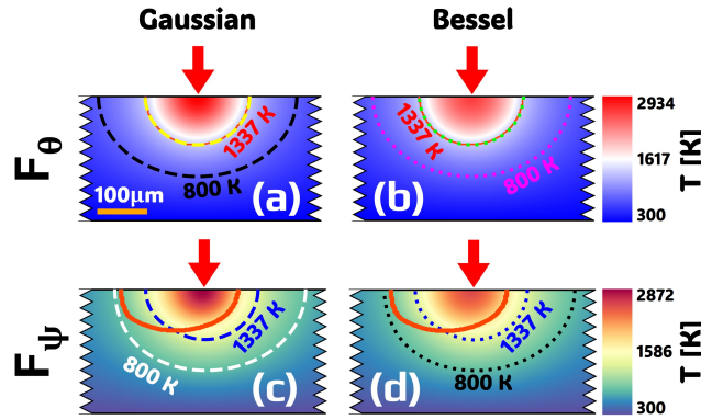
Figure A3: Visualization of thermal distribution across a cutout of simulation domain for Gaussian and Bessel laser sources. Plot (a) and (c) showcases the temperature profile for Gaussian heat source with driving force expression of F_\theta and F_\psi respectively. Similarly, (b) and (d) represents the temperature inside the computational domain with Bessel heat source for F_\theta and F_\psi correspondingly. A subtle difference in temperature profile can be noticed between Gaussian and Bessel based simulation results with a higher concentration of temperature distribution at the beam centre for Gaussian beam, the peak temperature reached by the domain under Bessel beam are found to be 2613.11 \text{ K} in (b) and 2548.95 \text{ K} in (d).
