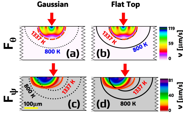
Figure A2: The illustration of velocity profile inside the meltpool when the laser heat source traverses to the domain midpoint at 12.5s into the simulation. Subplot (a) and (c) are associated with simulation under the Gaussian heat source for free energy expression of F_\theta and F_\psi respectively. The peak flow velocity for in the LIQUID phase for (a) and (c) are 119 \mu\text{m/s} and 75.61 \mu\text{m/s} respectively. In (b) and (d), the flow profile for simulation conducted under the Flat-Top heat source for F_\theta and F_\psi is presented. Although visually the velocity profile between results from Gaussian and Flat-Top laser beam lookalike there exists a smaller difference in numerical value of peak meltpool flow velocity reached at the illustrated time stamp with 114.47 \mu\text{m/s} and 81 \mu\text{m/s} for Flat-Top laser induced flow for F_\theta and F_\psi respectively.
