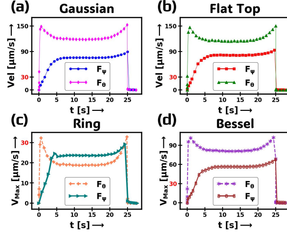
Figure 11: Subplots showing the evolution of maximum meltpool velocity during simulation for different laser beam profiles and free energy expressions. In (a), the Gaussian beam produces a higher peak velocity with F_\theta (magenta line with diamond markers) than with F_\psi (blue line with circular markers), averaging 123.75 \mu\text{m/s} and 71.76 \mu\text{m/s} , respectively. A similar trend is seen for the Flat-Top beam in (b), with average peak velocities of 119.94 \mu\text{m/s} ( F_\theta ) and 76.86 \mu\text{m/s} ( F_\psi ). In contrast, for the Ring beam ((c)), F_\psi yields slightly higher flow ( 22.65 \mu\text{m/s} ) than F_\theta ( 20.37 \mu\text{m/s} ). For the Bessel beam ((d)), the trend reverts to higher values with F_\theta ( 84.65 \mu\text{m/s} ) compared to F_\psi ( 52.39 \mu\text{m/s} ). Note that the y-axis scale differs in (c) and (d) to account for the lower velocity range; a red marker at 30 \mu\text{m/s} is included across all subplots for reference.
